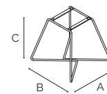
04 Base in tondino - Accessori: piedini, viti per piano Metal rod base - Accessories: glides, tabletop fixing screws
